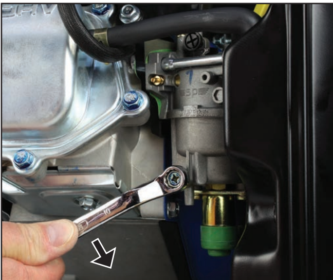
Figure 57 – Removing the Carburettor Drain Screw (WHXC5000, WHXC7000, WHXC8500E, WHXC8500E-PRO & WHXC8500E-AS II)
